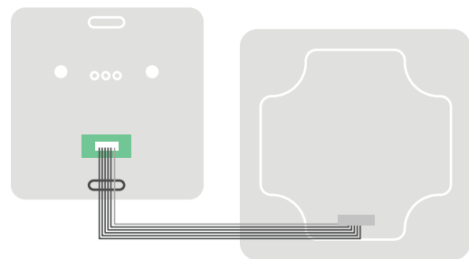
Touch panel and "W" module connection (W-2ONOFF; W-1SHUTT; W-2VLESS; W-INPKEY).
